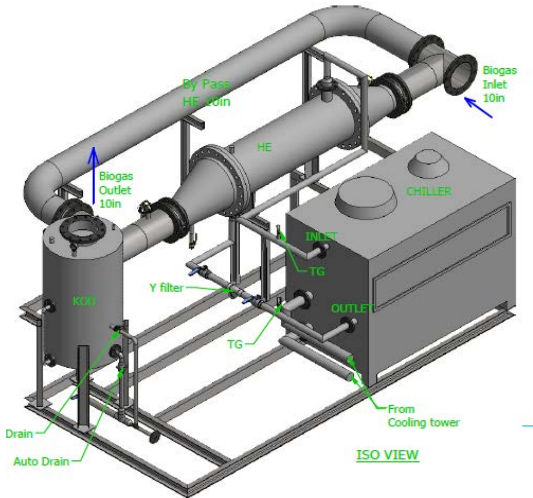
BD series with bypass line
